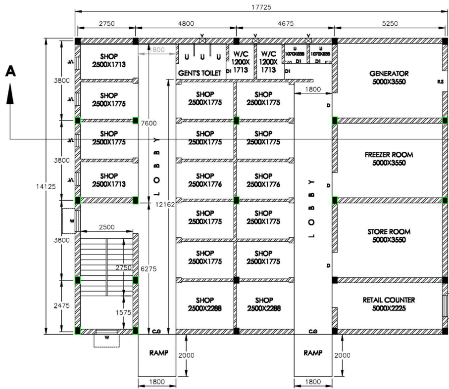
GROUND FLOOR PLAN NALBAN FISH MARKET
